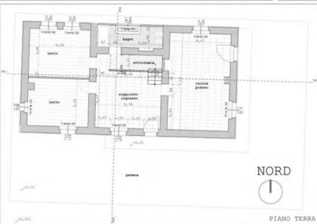
PIANO TERRA
