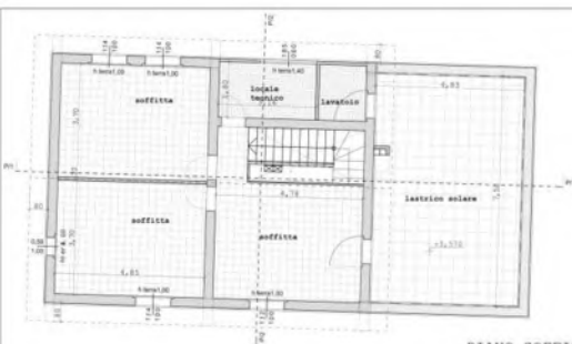
PIANO SOFFITTA
